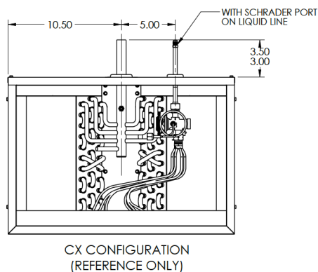
PERFORMANCE & DIMENSIONAL DATA (In.) - FIGURE 1
