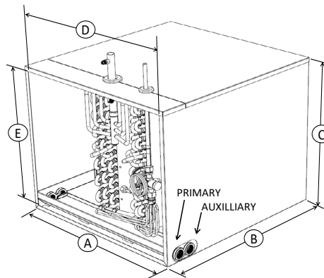
PERFORMANCE & DIMENSIONAL DATA (In.) - FIGURE 1
