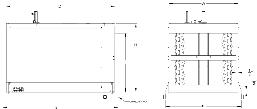
PERFORMANCE & DIMENSIONAL DATA (In.) - FIGURE 1
