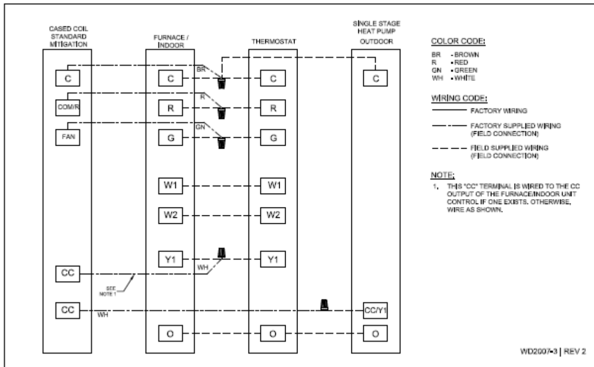
Single Stage Heat Pump
