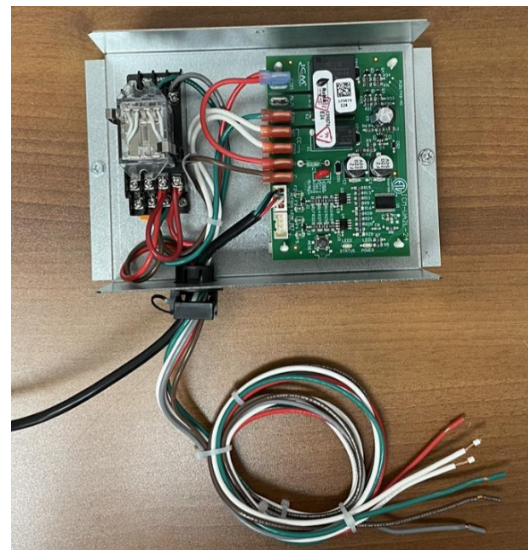
Standard + Accessory Control – Option “R”
