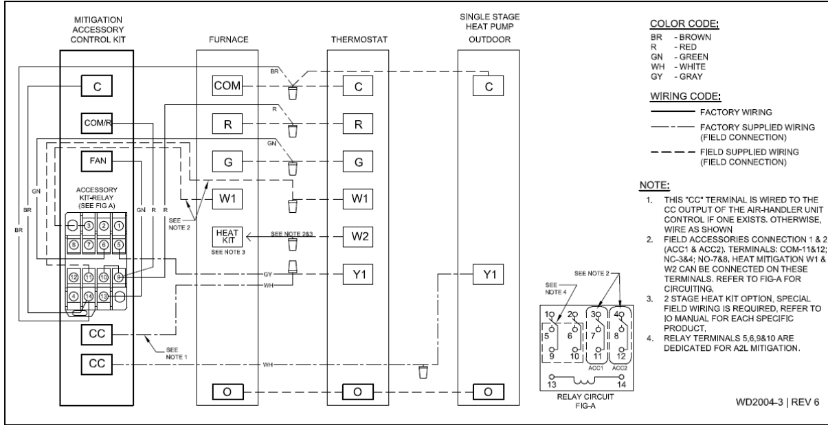
Single Stage Heat Pump
