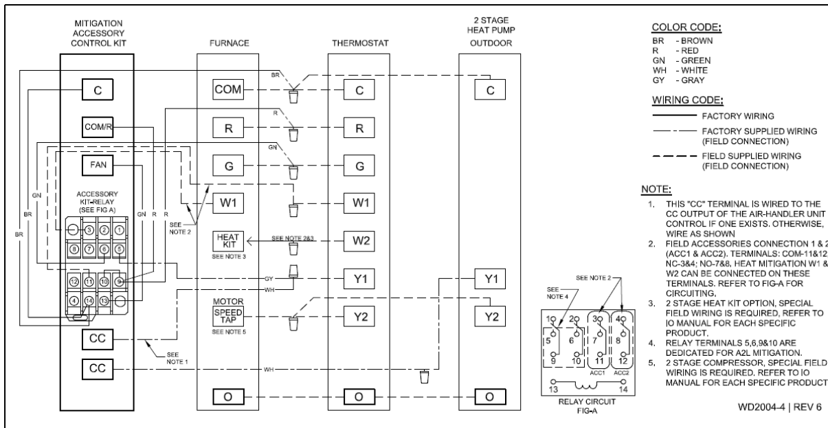
2 Stage Heat Pump
