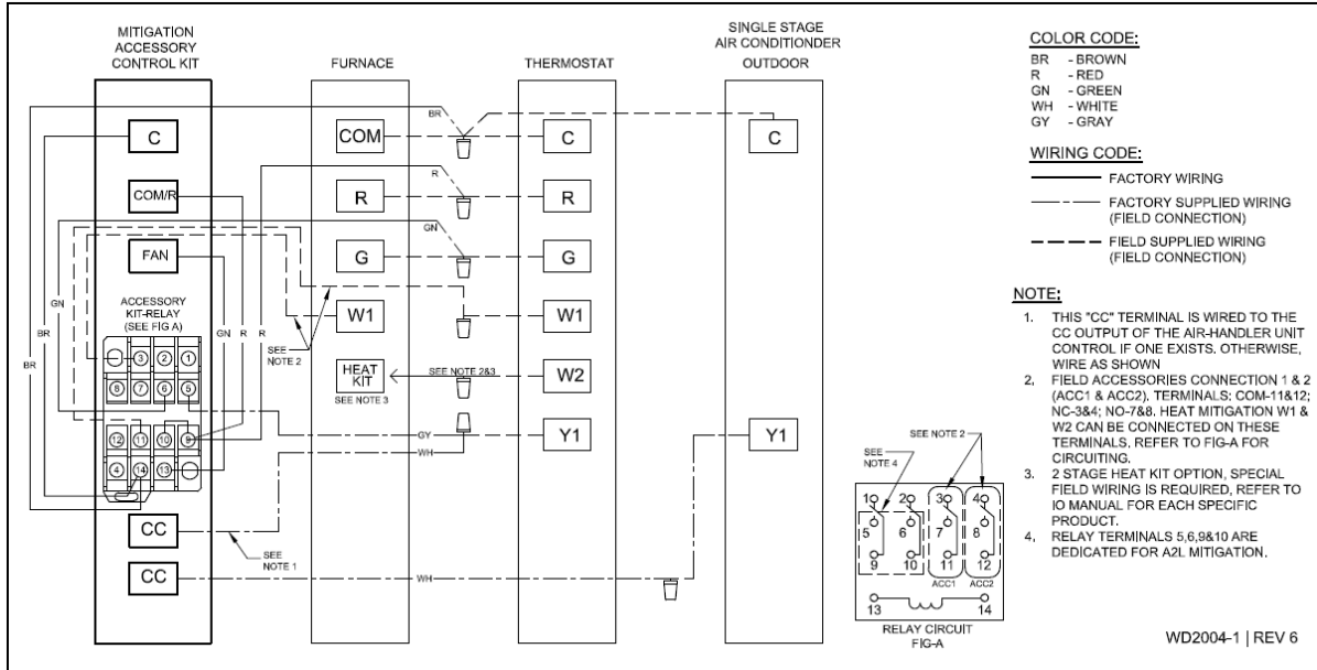
Single Stage Air Conditioner
