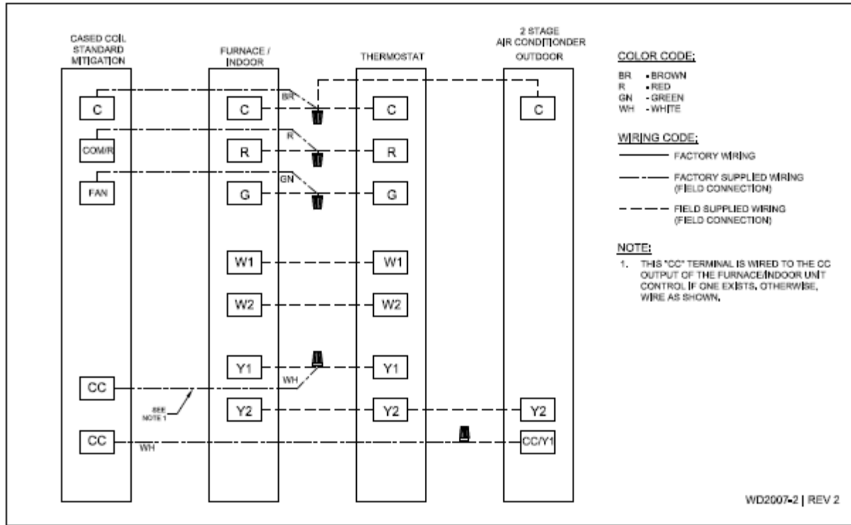
2 Stage Air Conditioner
