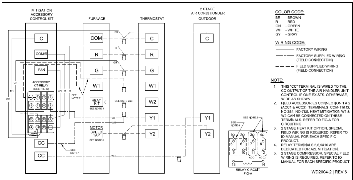
2 Stage Air Conditioner
