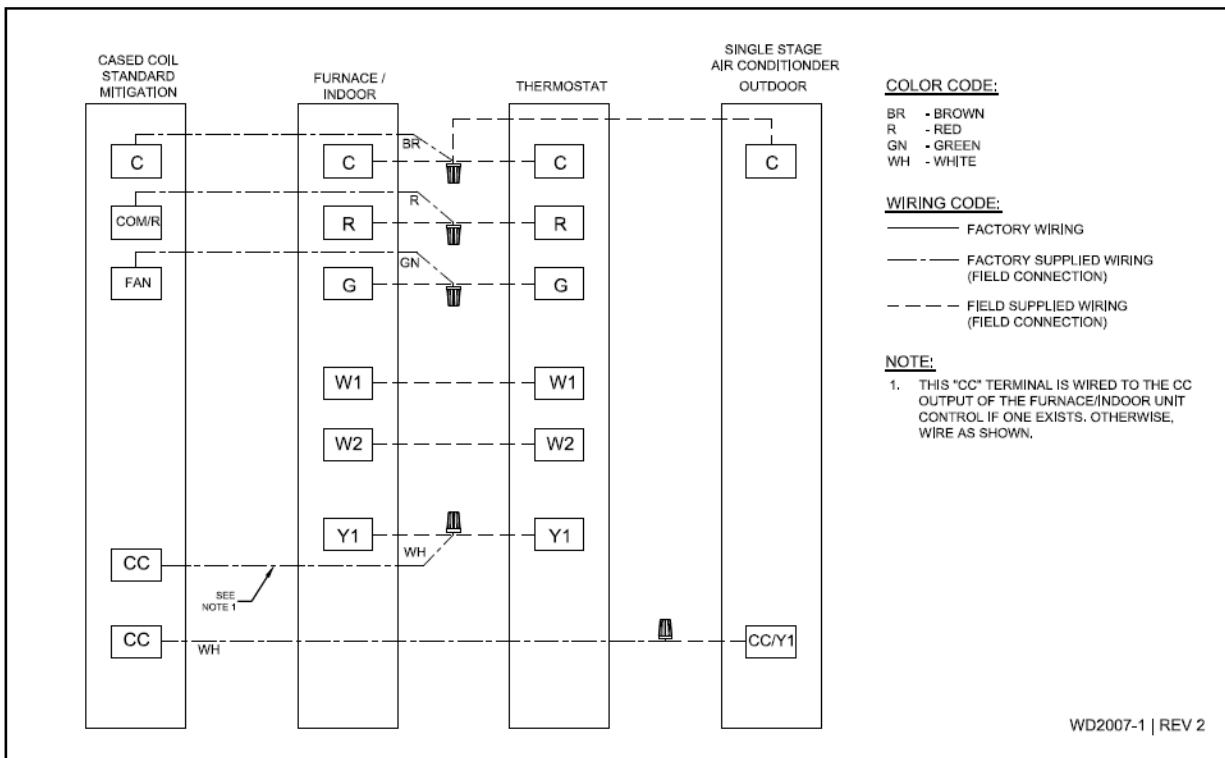
Single Stage Air Conditioner
